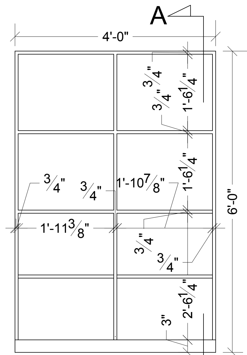
ELEVATION WITHOUT PANELS
