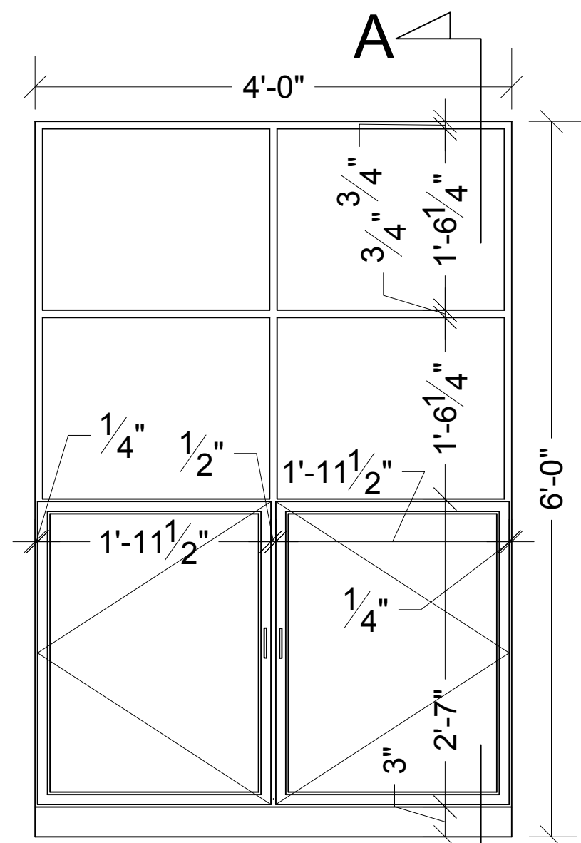
ELEVATION WITH PANELS
